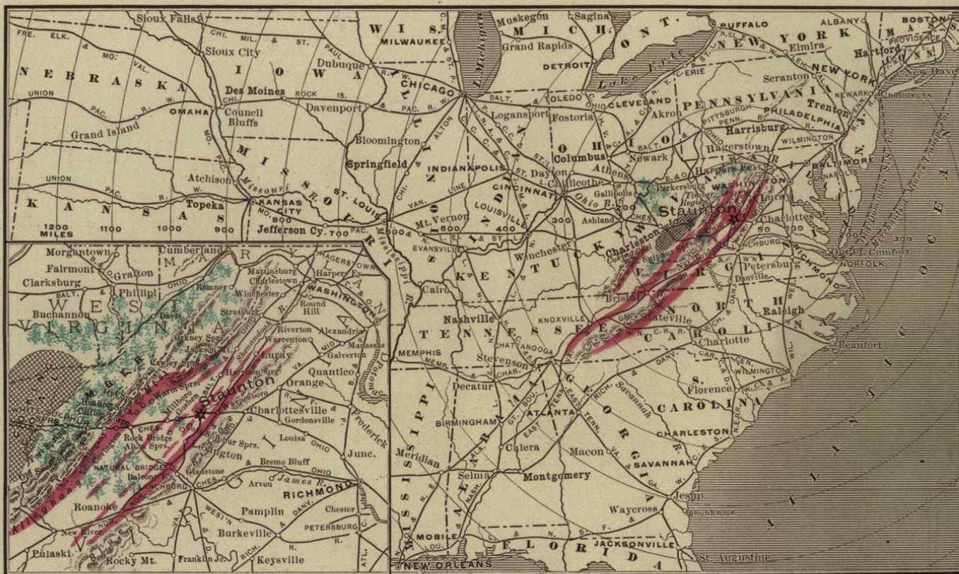
MAP SHOWING STAUNTON, VA., AND SURROUNDINGS.
